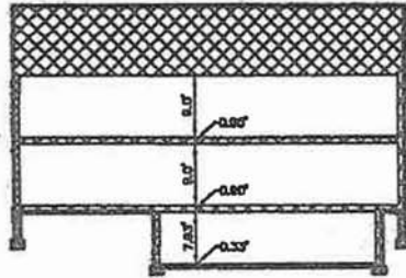
LONGITUDINAL SECTION B-B BUILDINGS #3, #4, #5
