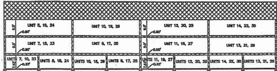
LONGITUDINAL SECTION A-A BUILDINGS #3, #4, #5
