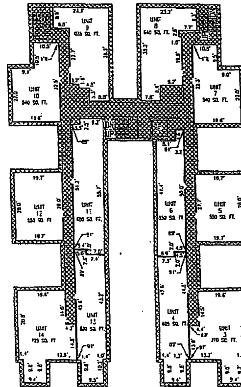
SEWARD AVE. (80 FT. WIDE) FIRST FLOOR PLAN
