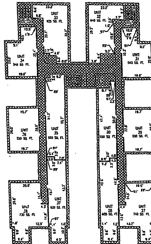
SEWARD AVE. (80 FT. WIDE) THIRD FLOOR PLAN
