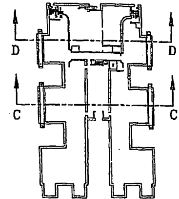
GROUND FLOOR PLAN SCALE 1"=20'
