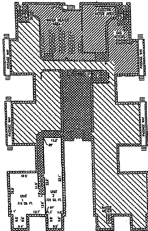
SEWARD AVE. (80 FT. WIDE) GROUND FLOOR PLAN
