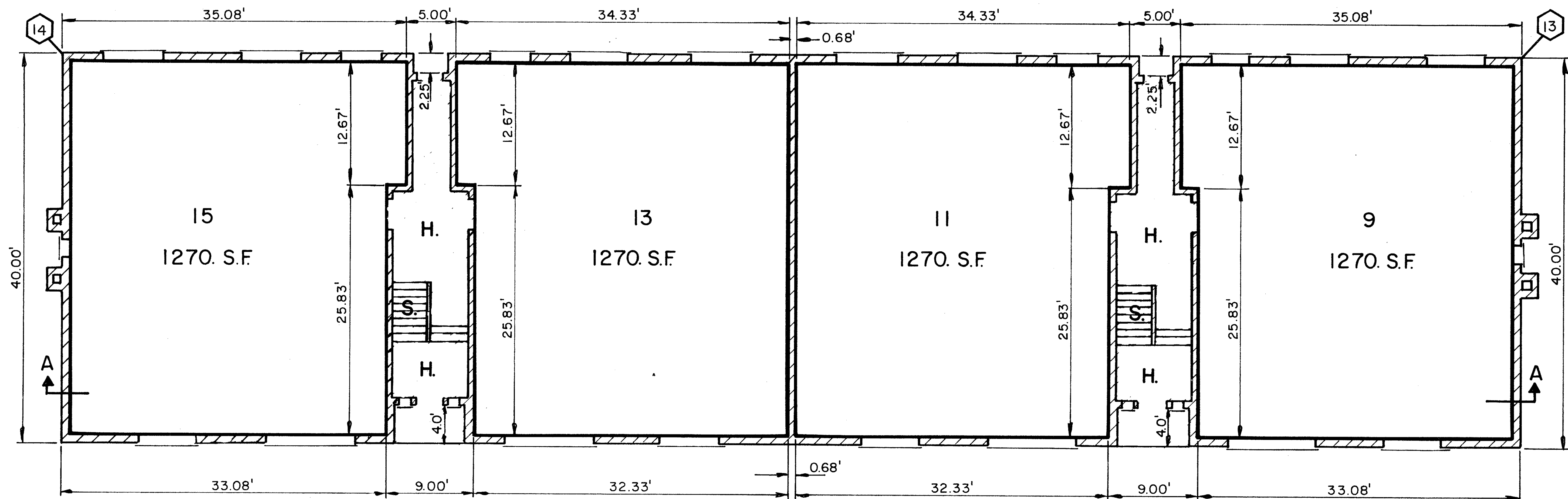
FIRST FLOOR PLAN BUILDING B
