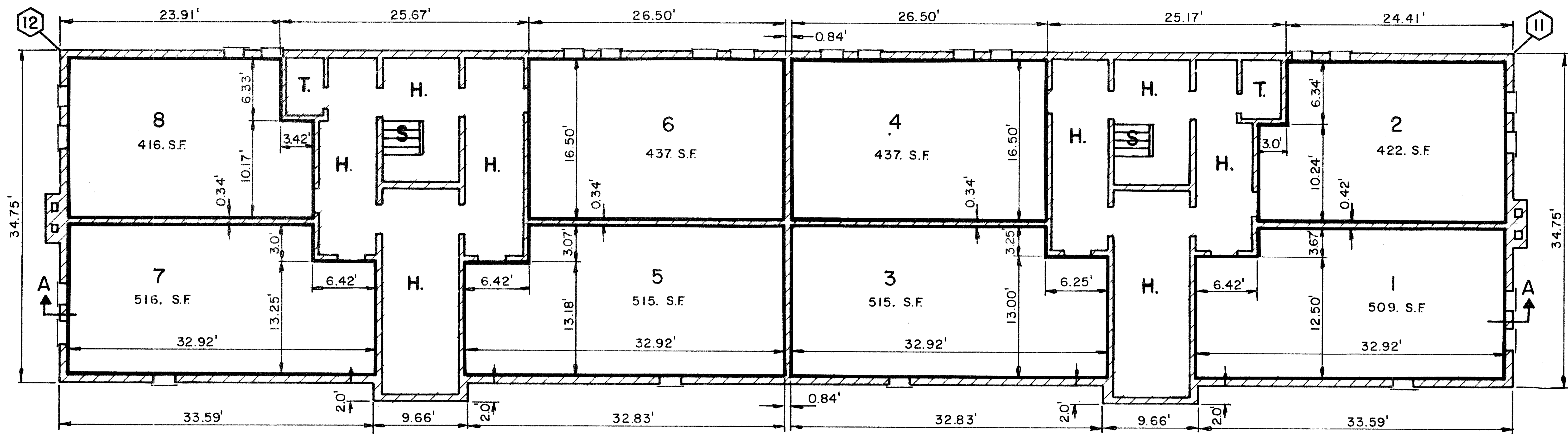
BASEMENT PLAN BUILDING A
