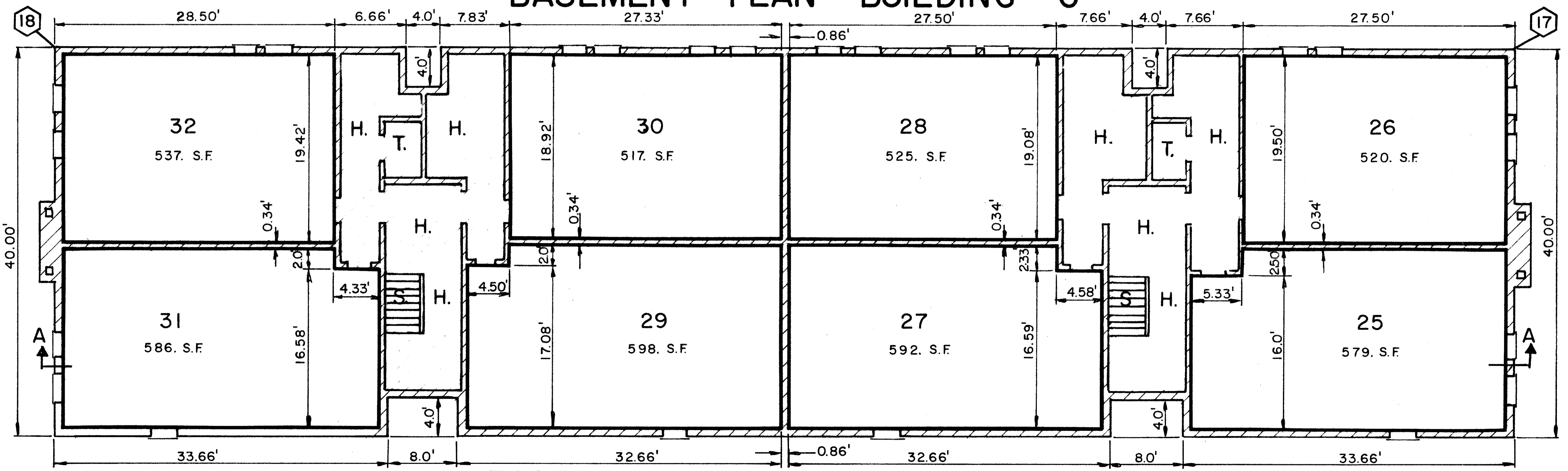
BASEMENT PLAN BUILDING D
