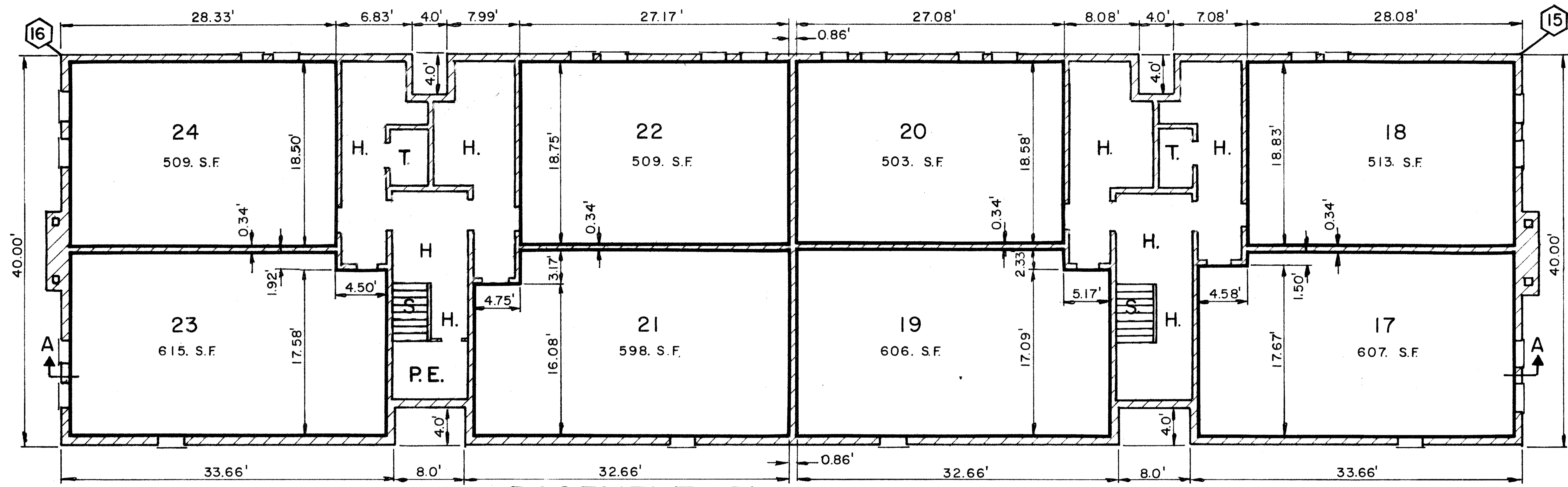
BASEMENT PLAN BUILDING C
