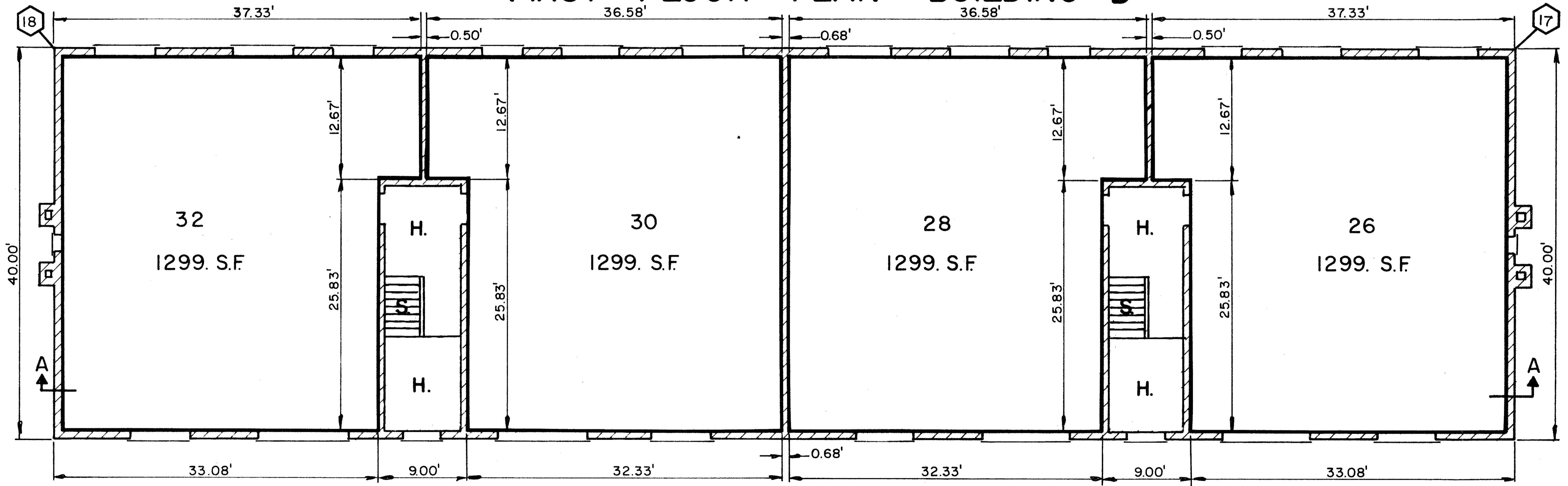
SECOND FLOOR PLAN BUILDING D
