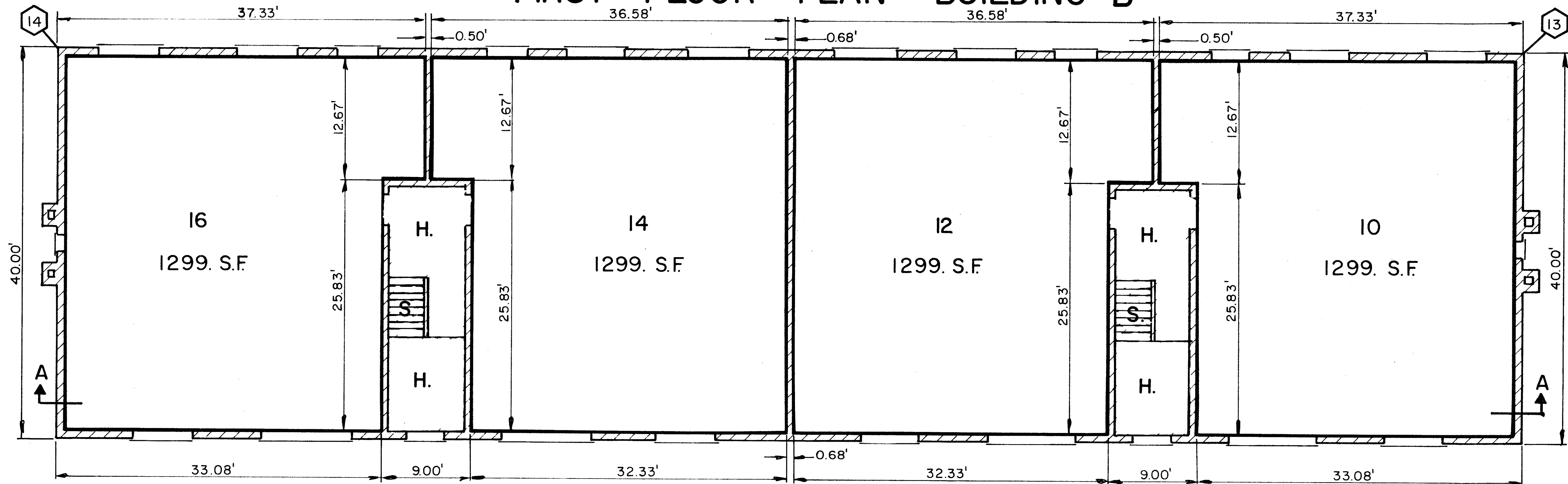
SECOND FLOOR PLAN BUILDING B
