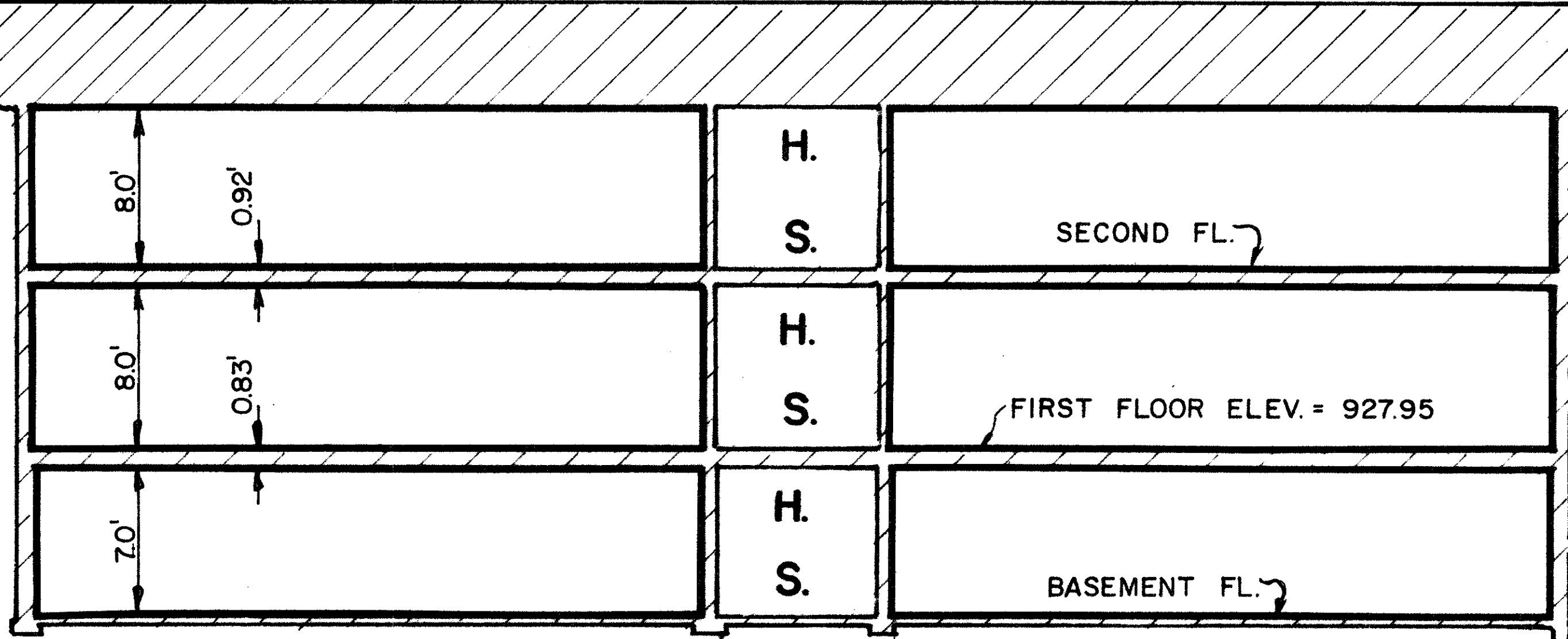
CROSS SECTION A-A BUILDING E.
