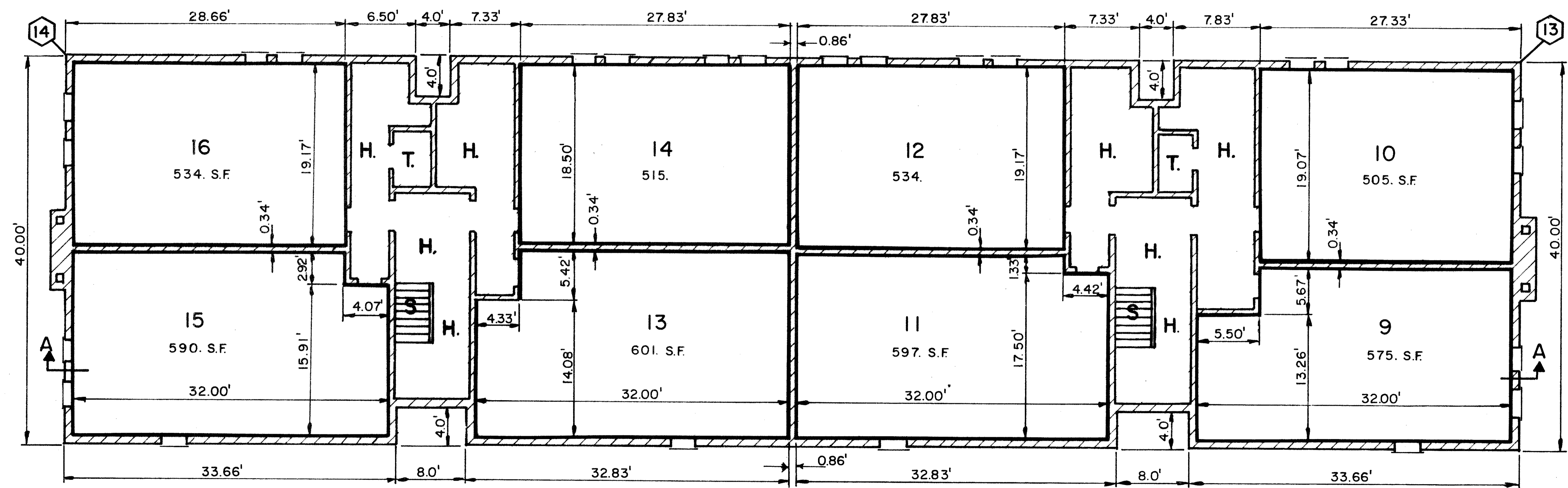
BASEMENT PLAN BUILDING B
