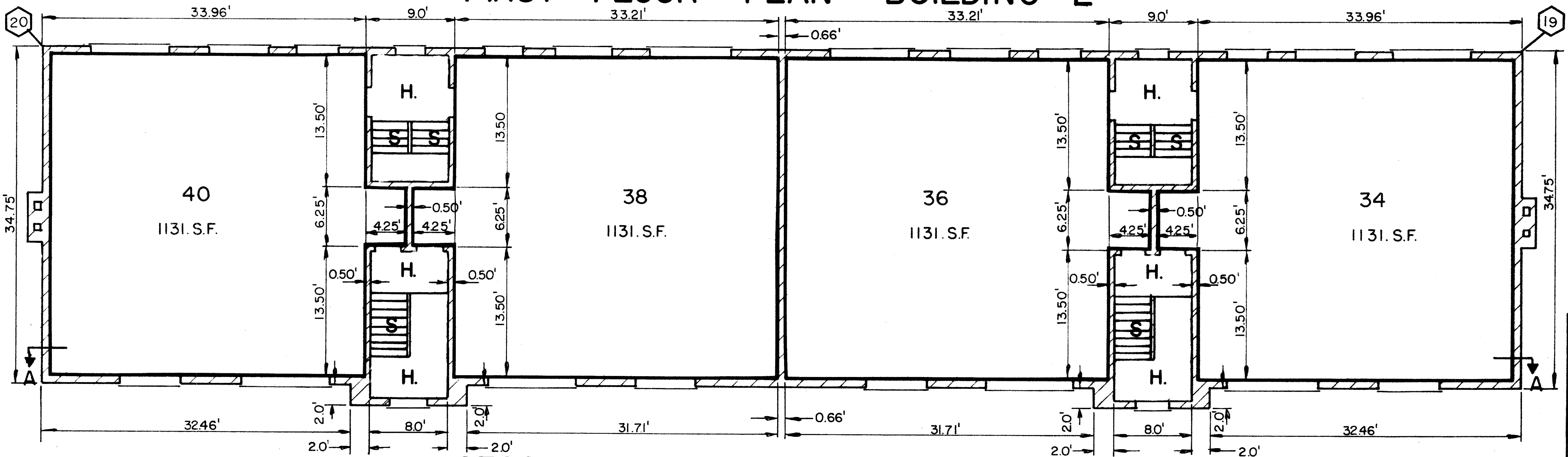
SECOND FLOOR PLAN BUILDING E
