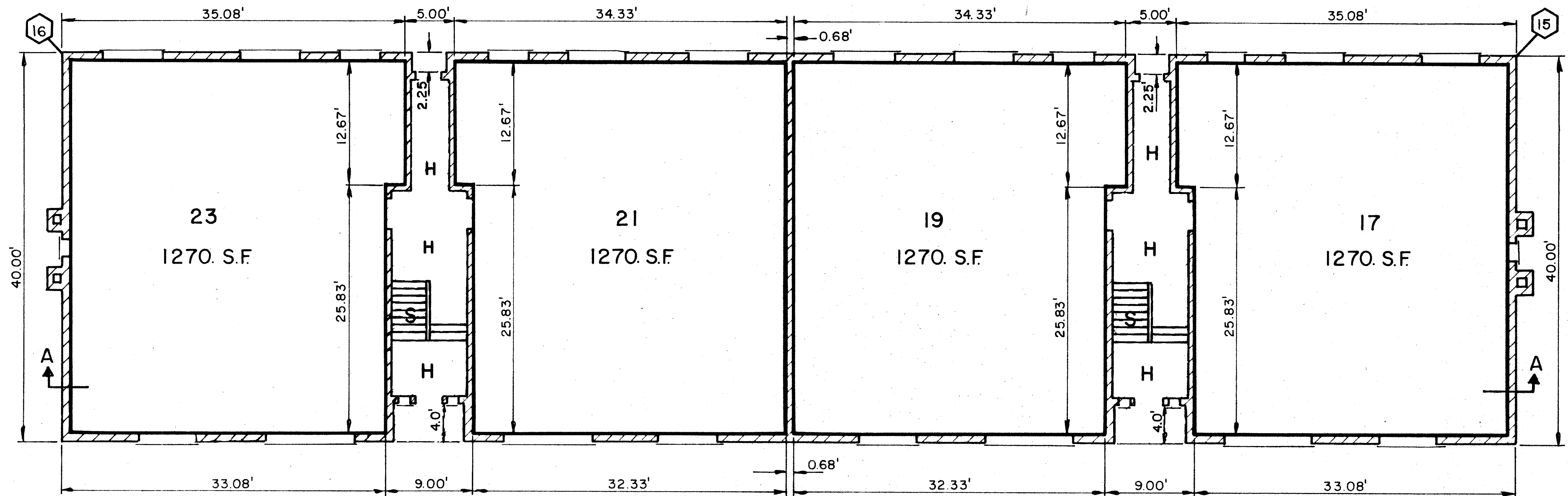
FIRST FLOOR PLAN BUILDING C
