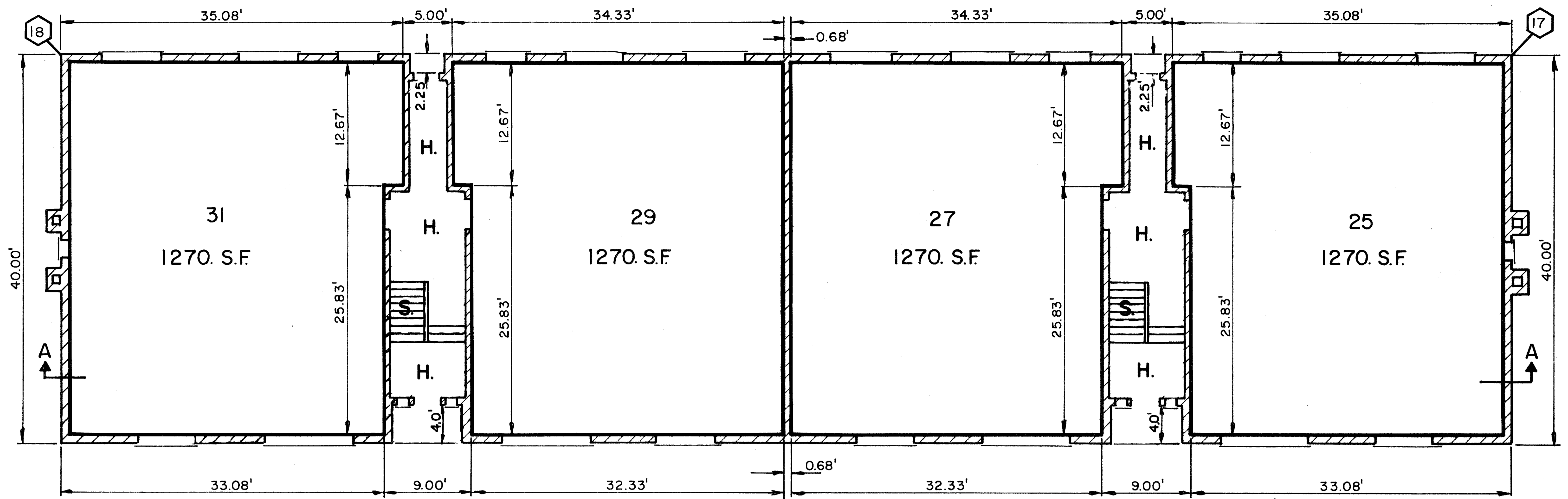
FIRST FLOOR PLAN BUILDING D
