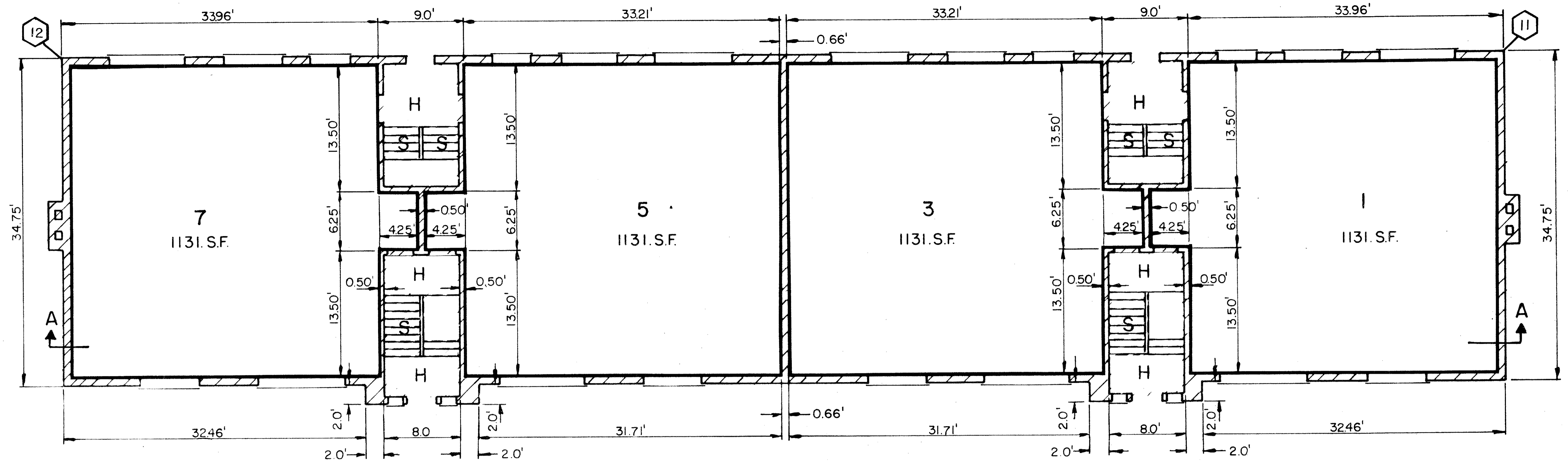
FIRST FLOOR PLAN BUILDING A
