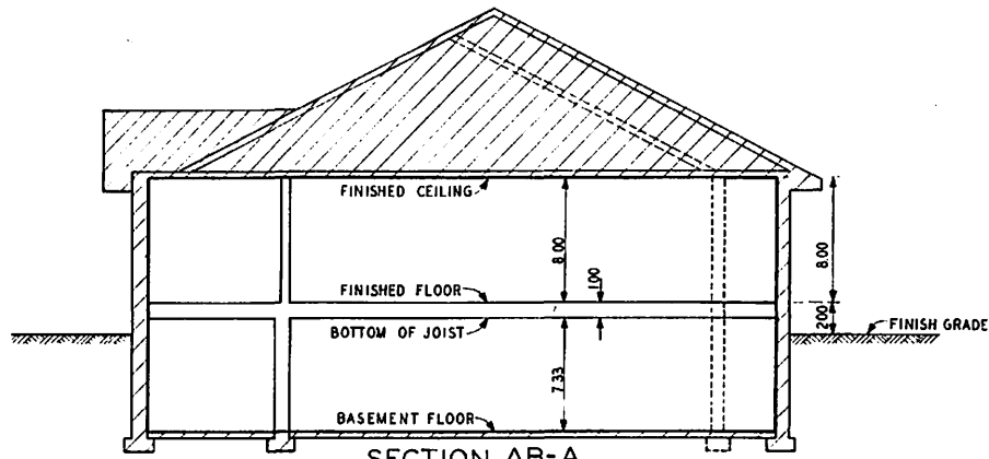
SECTION AB-A
