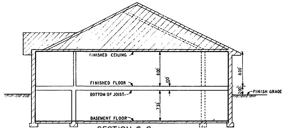
SECTION C-C
