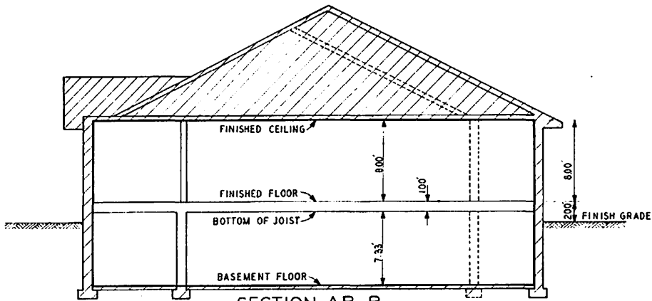
SECTION AB-B
