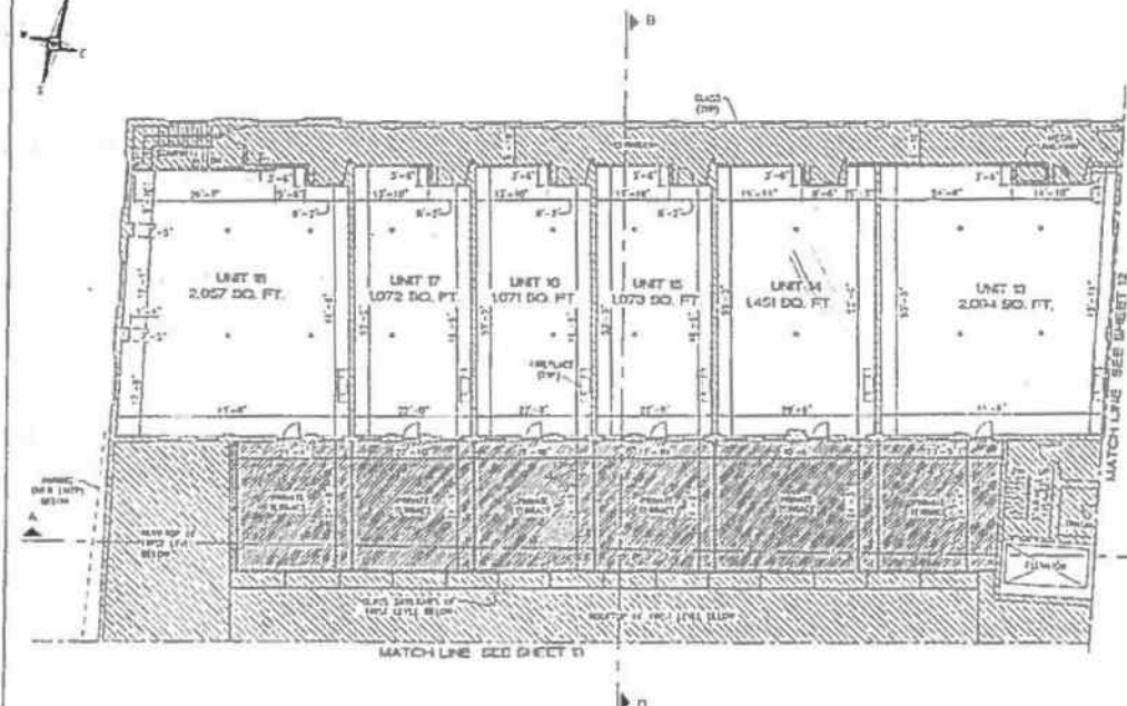
SECOND LEVEL PLAN - UNITS 13, 14, 15, 16, 17, 18
