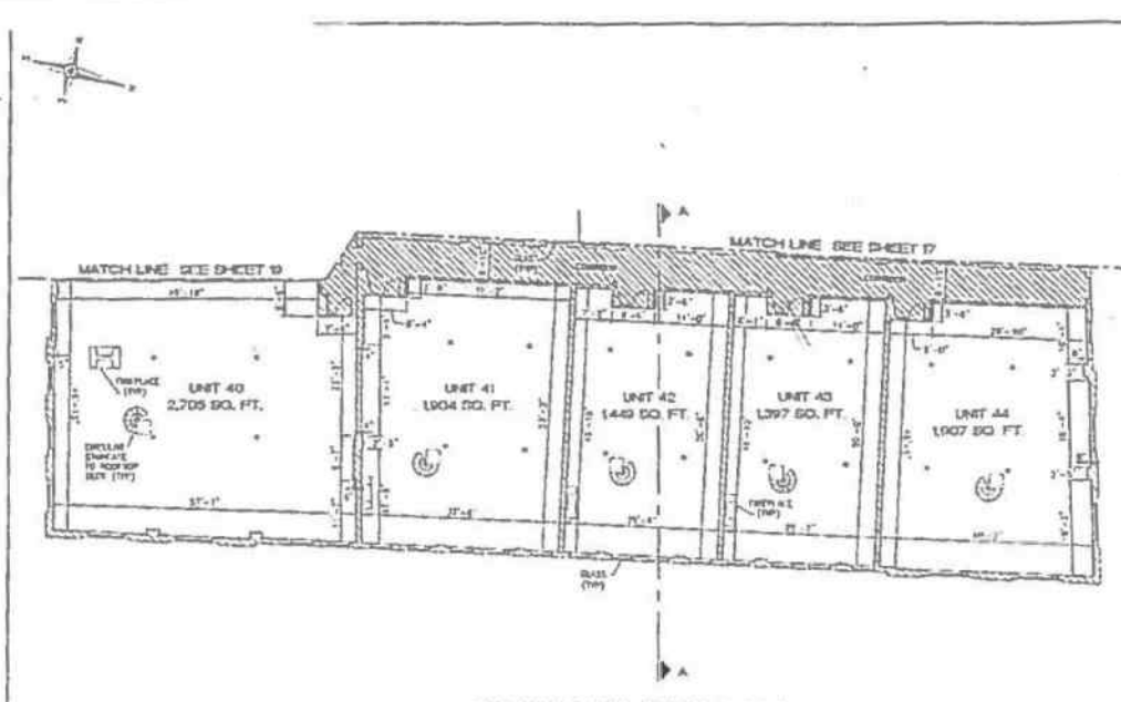
FOURTH LEVEL PLAN - UNITS 40, 41, 42, 43, 44
